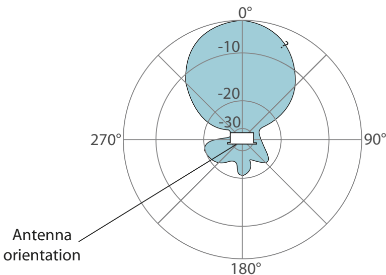
H-plane Azimuth pattern
